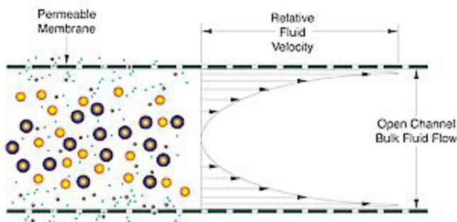
Tangential Flow Pattern in Vibratory VSEP Membrane Systems
